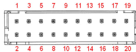
Signal Output Signal Connectors (SK2)
