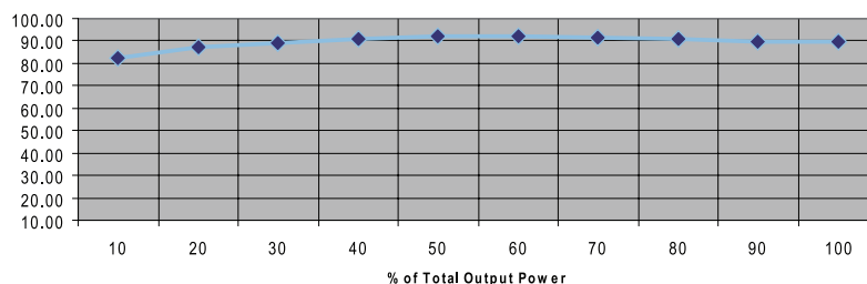
230 Vac Efficiency
