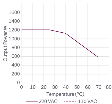
Temperature Derating Curve UX6
