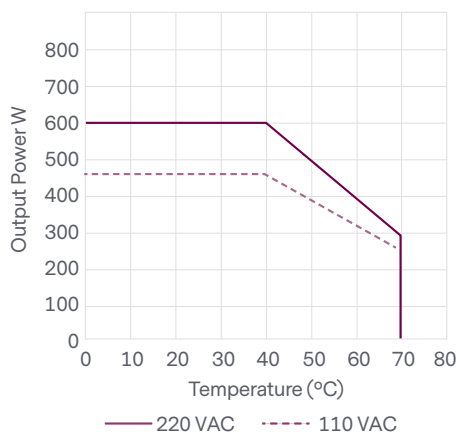
Temperature Derating Curve UX4
