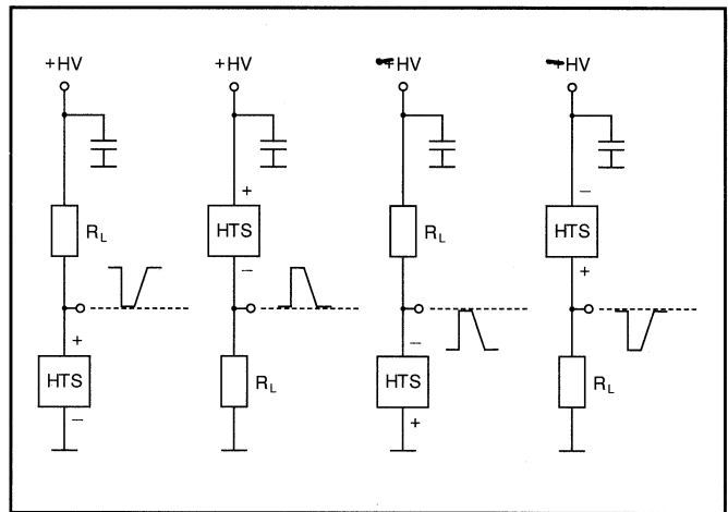
Fig. 6: Basic Circuit Configurations
