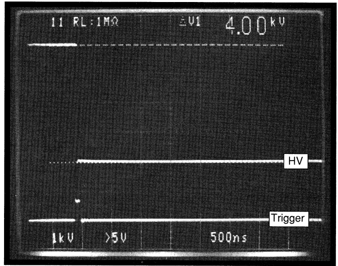
Fig. 2c: Pulse Shape, R_L = 1MOhm ; C_L = 30pF ; 1kV/div.
