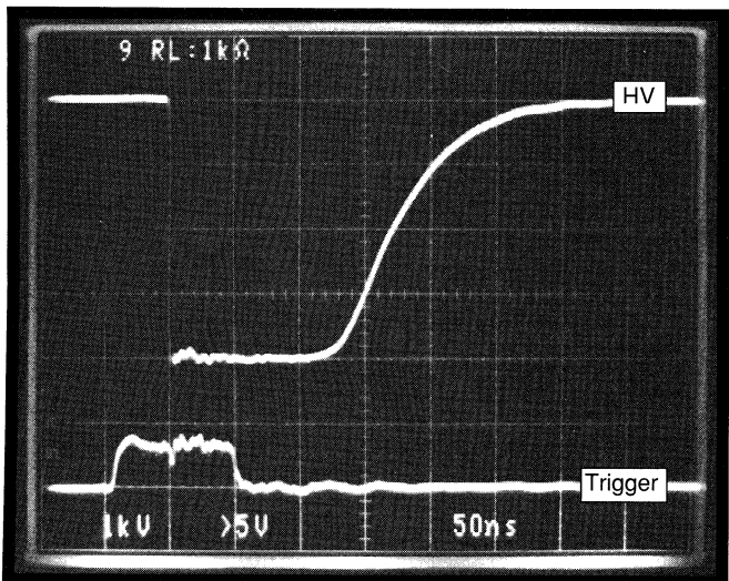
Fig. 2b: Pulse Shape, R_L = 1k\Omega ; C_L = 30pF ; 1kV/div.
