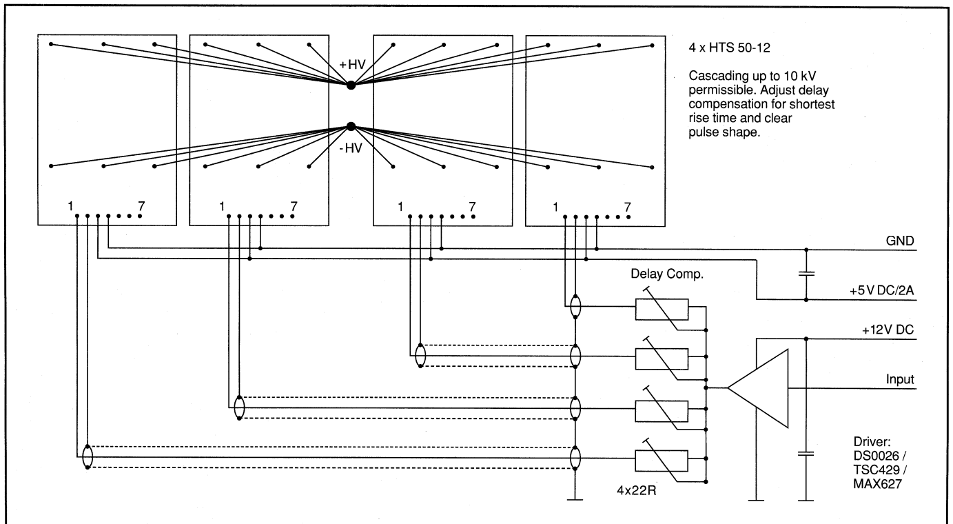
Fig. 4: Paralleling HTS 50-12
