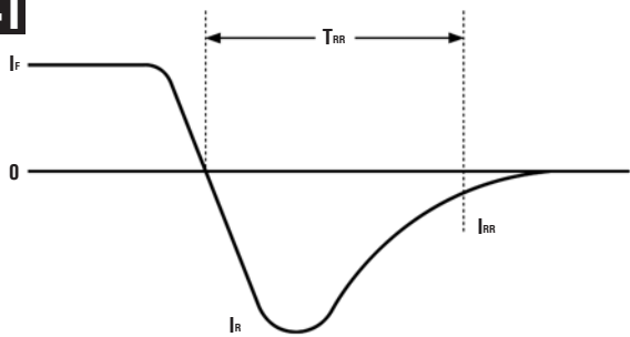
Reverse Recovery Measurement Waveform
