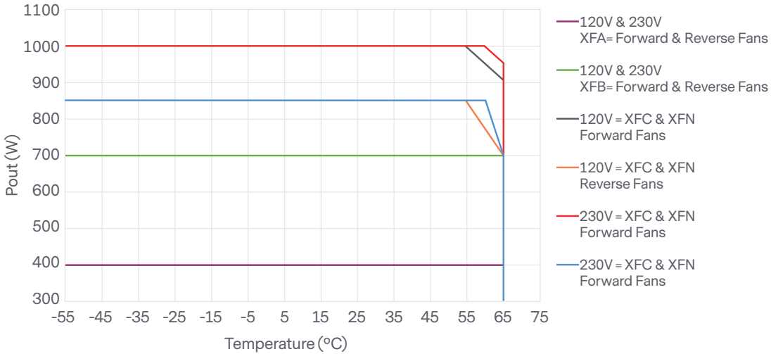
Temperature Derating Curve for XF Models
