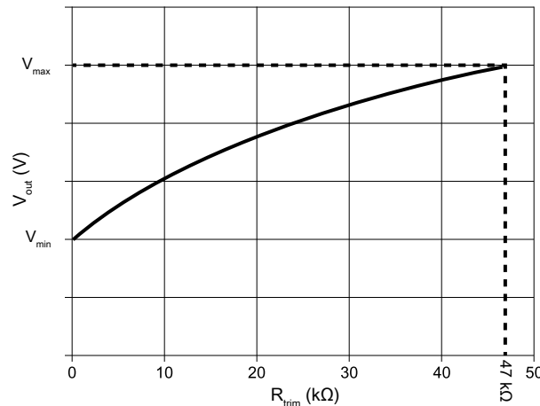
Figure 6-19. R_{\text{trim}} versus V_{\text{out}}
