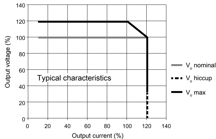
Figure 6-26. Current and power overload characteristics
