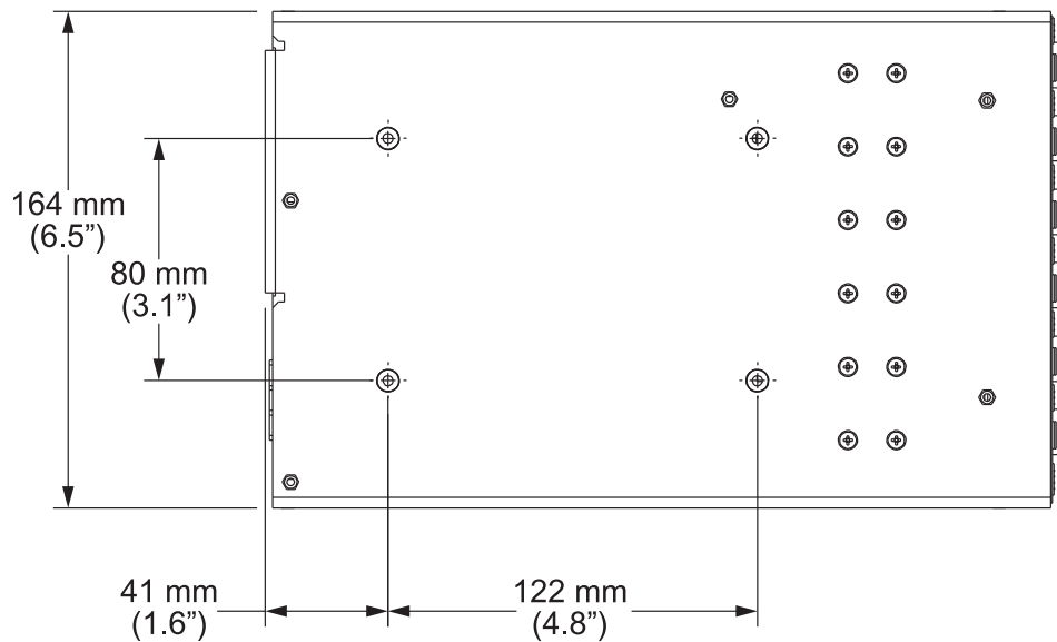
Figure 6-4. CoolX unit dimensions, bottom view
