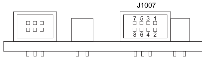
Figure 5-1. J1007 system signal connector
