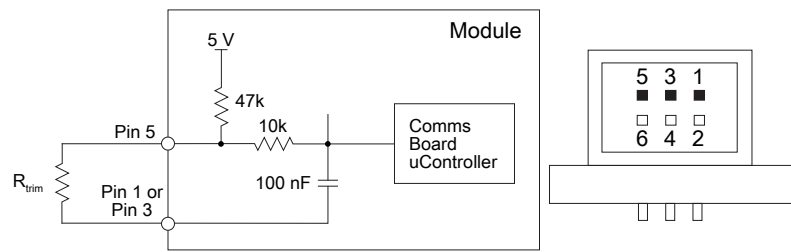
Figure 6-23. CoolMod wiring diagram for remote current setting using external resistance
