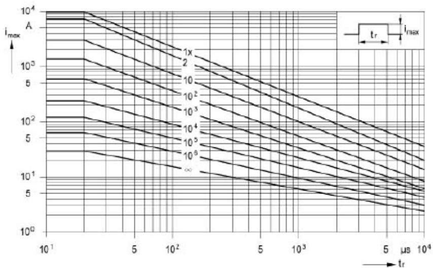
DERATING CURVE
