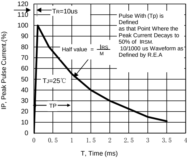
Fig. 3 - Pulse Waveform
