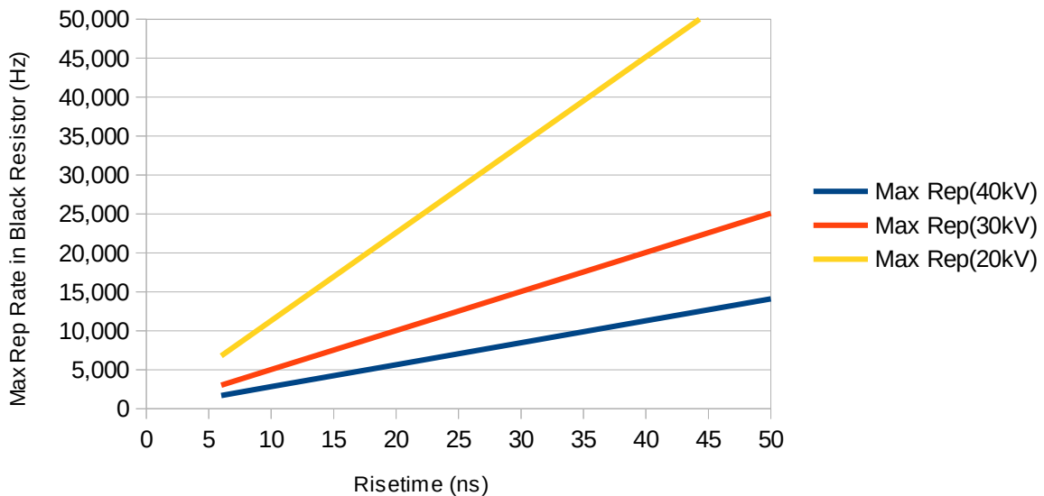
Max Rep Rate PVM-1, PVM-2, PVM-3 With Black Damping Resistor
