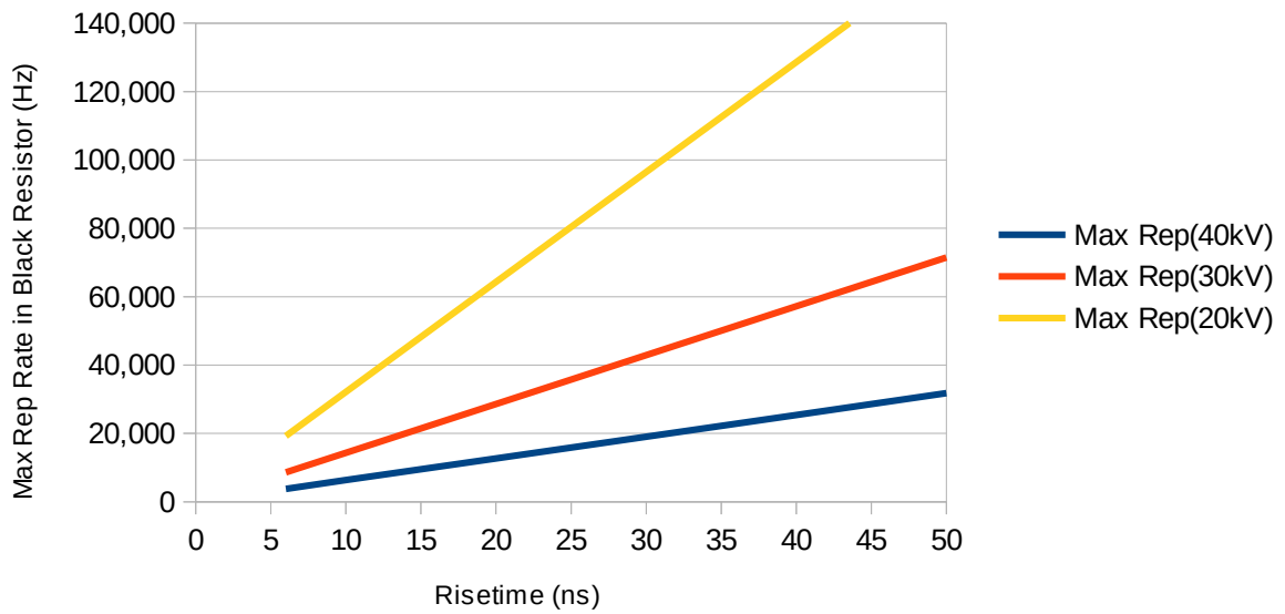
Max Rep Rate PVM-5, PVM-6 With Black Damping Resistor
