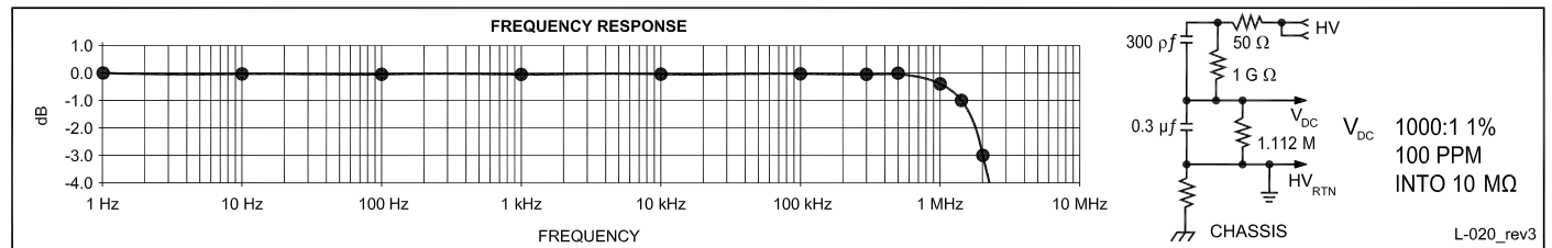
Fig. E - Bandwidth and equivalent circuit (compensated divider)
