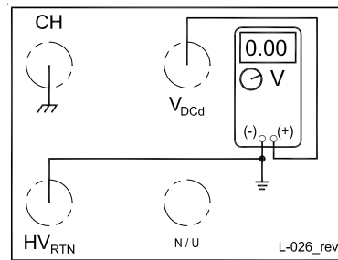
Fig. B - Electrical connections (precision divider)
