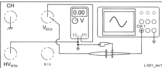
Fig. F - Electrical connections (compensated divider)
