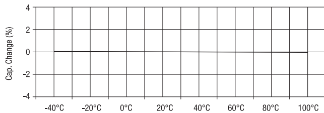
NP0 Typical Temperature Characteristics Curve
