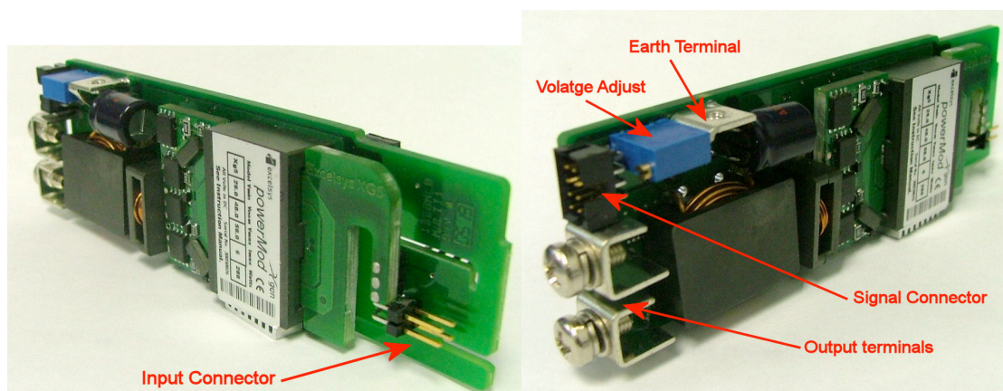
Fig 2: PowerMod description
