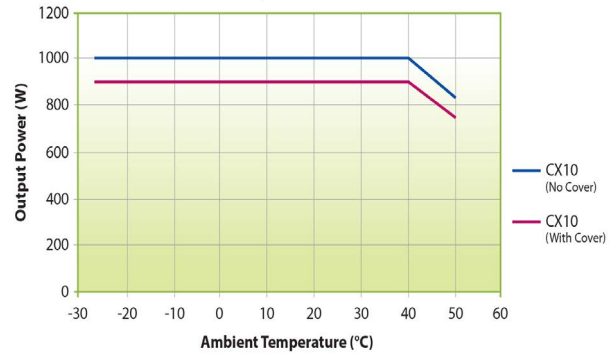
CX10 Temperature Derating Curves - IEC Input Connector
