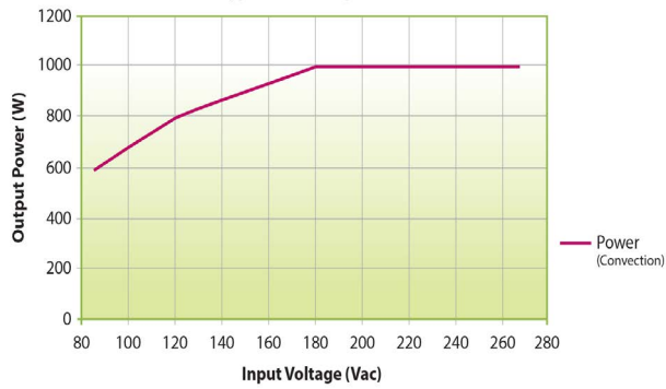
CX10 Input Voltage Typical Derating Curve
