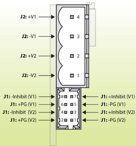
C_mG & C_mH Output Connectors
