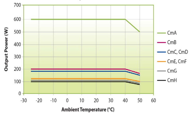
CoolX1000 Cm Typical Derating Curves - IEC Input Connector
