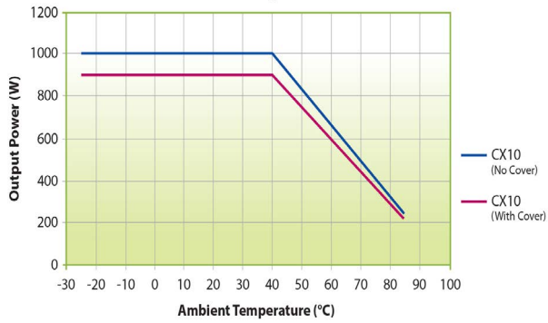
CX10 Temperature Derating Curves - Screw Terminal Input Connector
