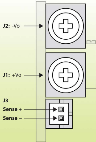
CmA, C_mB, C_mC, C_mD Output Connectors
