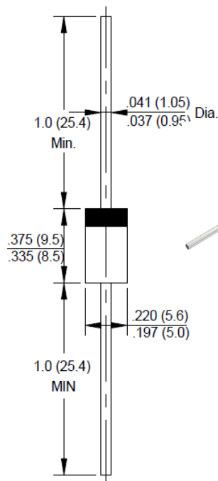
Package Outline Dimensions in Inches (Millimeters)
