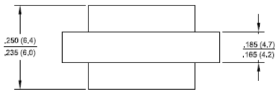
Package Outline Dimensions in Inches (Millimeters)
